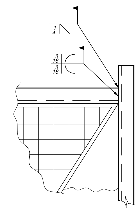
DETAIL '1'
